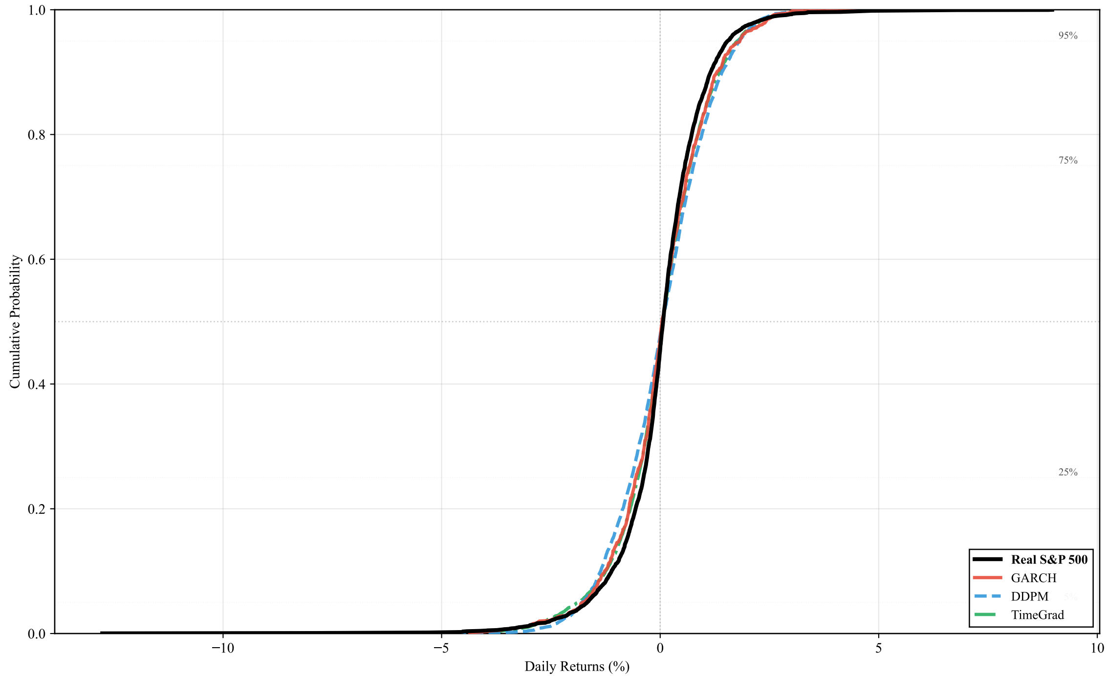
Cumulative Distribution Function Comparison (Baseline Models)
